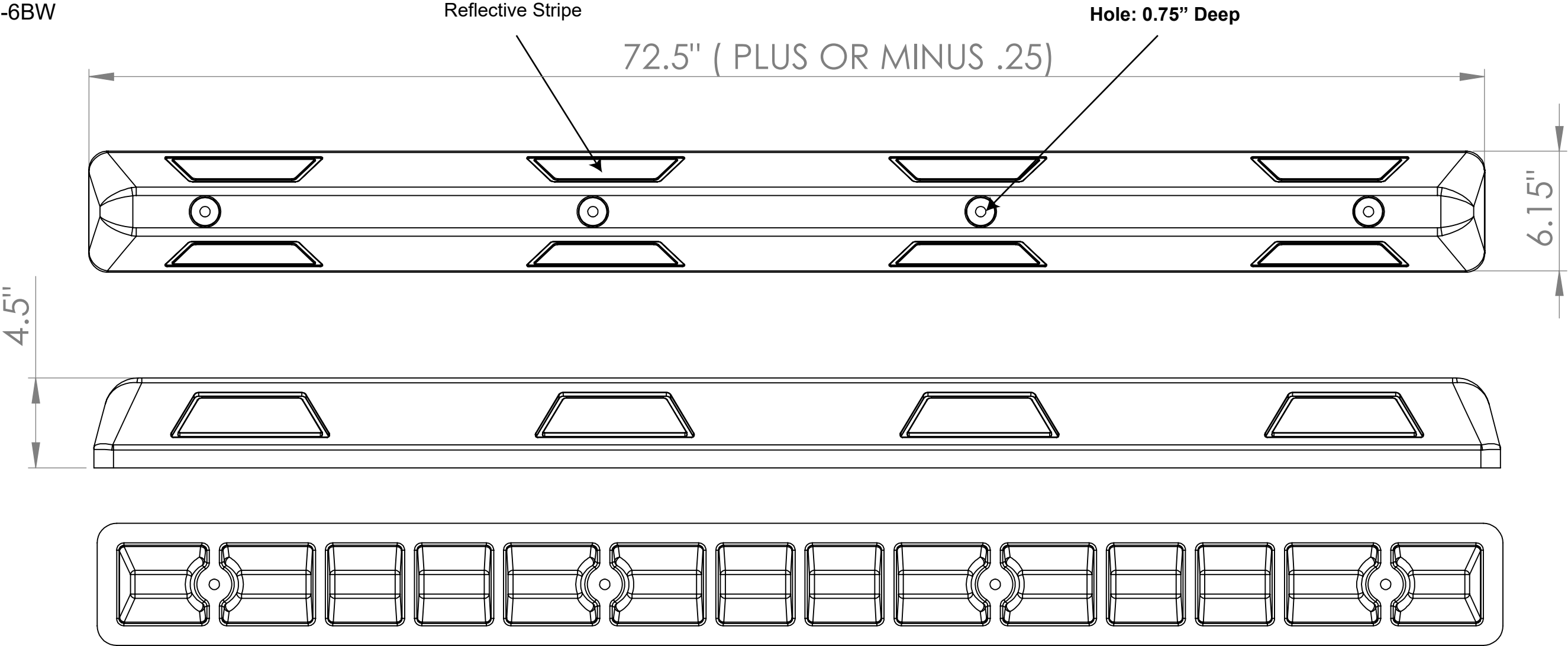
BOTTOM VIEW
